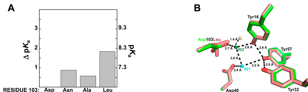
Figure 6. Effects of Asp103 mutations on the Tyr pK_a . (A) \Delta pK_a values relative to the pK_a value of Asp40Asn. The values are from Table 2. (B) Superposition of structural models of Met116Ala (green, PDB ID 3RGR) and Asp103Leu (salmon, PDB ID 1W00) suggests the position of an organized water molecule in the oxyanion hole is perturbed in Asp103Leu (salmon sphere) compared to wild type (green sphere). Wat1 is not observed in the Asp103Leu structure.
