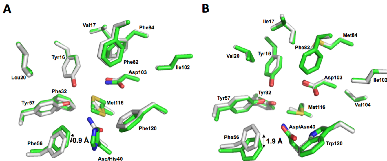
Figure 12. Introduction of charged residues at position 40 cause structural rearrangements of Phe56 relative to Asp40Asn. (A) Superposition of the 2.0 Å Asp40His/Asp103Asn structure determined herein (PDB ID 3MYT, carbon atoms colored green) and the previously determined 2.3 Å Asp40Asn structure (PDB ID 1QJG, carbon atoms colored white) showing that Phe56 is displaced 0.9 Å upon introduction of the His residue. (B) Superposition of the previously determined structures of the 1.1 Å wild-type KSI structure (PDB ID 1OH0, carbon atoms colored green) and the 2.0 Å Asp40Asn structure (PDB ID 1OGX, carbon atoms colored white) showing that the Phe56 side chain is displaced 1.9 Å upon changing residue 40 from Asp to Asn. pKSI numbering is used for simplicity.
