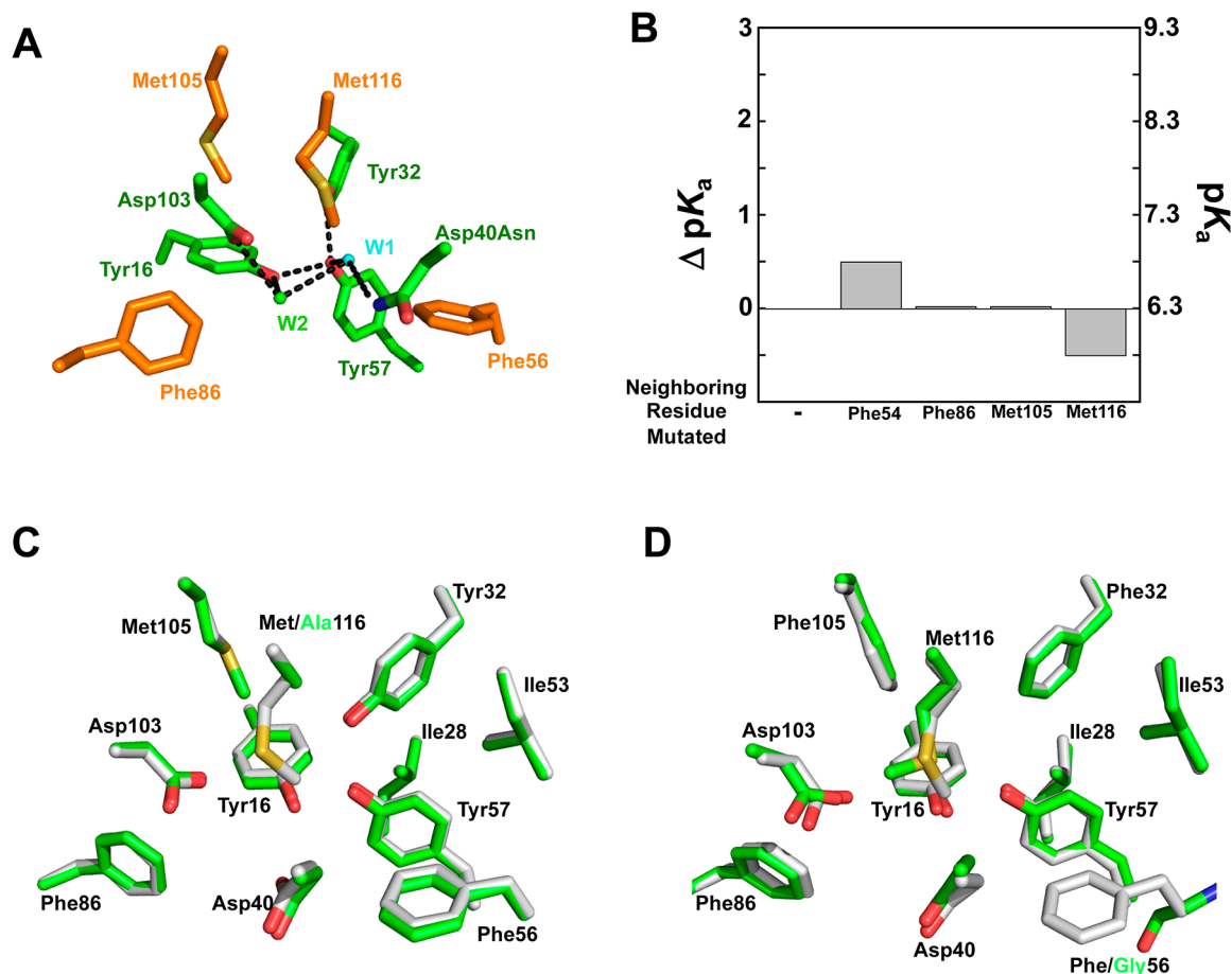
Figure 9. Effects of neighboring group mutations on the Tyr pK a . (A) Structural model showing the positions of residues neighboring the active-site hydrogen-bond network that have been mutated. The same model as in Figure 2C is shown but with peripheral residues added (orange). (B) Changes in pK a upon mutation of the peripheral residues to Ala relative to Asp40Asn KSI. “-” refers to the Asp40Asn variant. The values are from Table 7. (C) Structural overlays of the Met116Ala mutant (carbon atoms colored green) and wild-type pKSI (carbon atoms colored white). (D) Structural overlay of tKSI Phe56Gly mutant (carbon atoms colored green) with wild-type tKSI (carbon atoms colored white) showing that the residues engaged in the hydrogen-bonding network are essentially superimposable. pKSI numbering is used for tKSI for simplicity.
