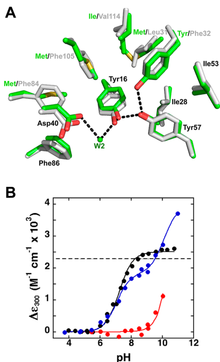
Figure 10. Recreating the potential hydrogen-bond network in tKSI. (A) Superposition of structural models of the wild-type pKSI (green, PDB ID 1OPY) and wild-type tKSI (gray, PDB ID 8CHO); although the active site residues are the same, the surrounding residues are different. (B) Relative extinction coefficients at 300 nm for pKSI D40N/D103N (black), tKSI D40N/D103N (red), and tKSI F32Y/D40N/D103N (blue) (pKSI numbering is used throughout). Absorbance spectra were collected as described in the Experimental Section. The lines are fits of the data to the ionization of one or two Tyr residues, and give Tyr pK_a values of 7.2 for pKSI D40N/D103N, >10 for tKSI D40N/D103N, and 7.3 for tKSI F32Y/D40N/D103N. The values are from Table 8.
