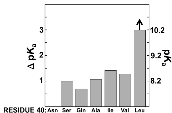
Figure 7. Effects of Asp40 mutations on the Tyr pK_a . The \Delta pK_a values are relative to the pK_a value of Asp40Asn/Asp103Asn and are from Table 3.
