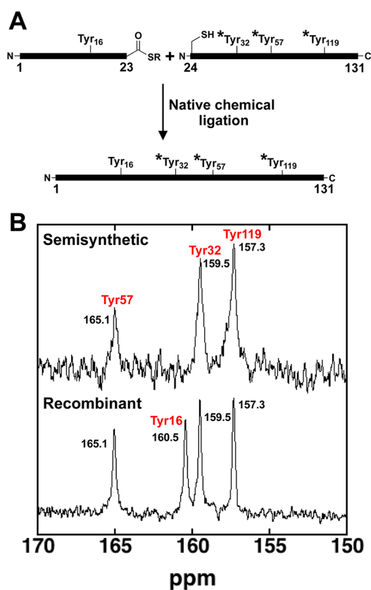
Figure 1. ^{13}\text{C} NMR spectra of site-specifically labeled semisynthetic R15K/D21N/D24C/D40N KSI to assign the identity of the ionizing Tyr residue. (A) Synthetic fragment (1–23) bearing unlabeled Tyr16 is ligated to a recombinant fragment (24–131) bearing ^{13}\text{C}_\alpha -Tyr at residues 32, 57, and 119 (*Tyr). (B) ^{13}\text{C} NMR spectrum for fully recombinant R15K/D21N/D24C/D40N KSI with ^{13}\text{C}_\alpha -Tyr residues and semisynthetic R15K/D21N/D24C/D40N KSI with unlabeled Tyr16. The spectrum of semisynthetic KSI lacks the peak at 160.5 ppm, allowing assignment of this peak to Tyr16. The peak at 157.3 ppm was previously assigned to Tyr119, and the peak at 165.1 was attributed to Tyr57, as described in the text.
