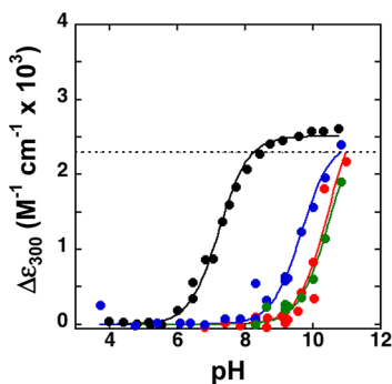
Figure 4. Changes in extinction coefficients at 300 nm relative to pH 4 for D40N/D103N (black), Y16F/D40N/D103N (red), Y32F/D40N/D103N (blue), and Y57F/D40N/D103N (green). Absorbance spectra were collected as described in the Experimental Section. The lines are a fit of the data to a titration curve and give pK_a values of 7.2 for D40N/D103N, >9 for Y32F/D40N/D103N, >10 for Y16F/D40N/D103N, and >10 for Y57F/D40N/D103N.
