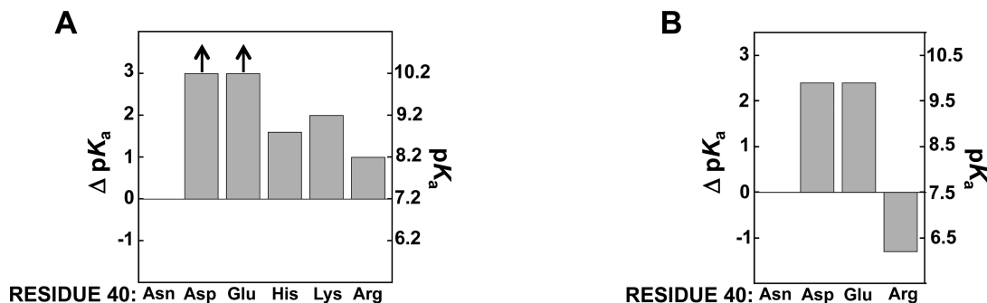
Figure 11. Effect of charged residues at position 40 on the Tyr pK_a . (A) Effects of charged residues in the Asn103 background. The \Delta pK_a values are relative to the pK_a value for Asp40Asn/Asp103Asn KSI. The values are from Table 9. (B) Effects of charged mutations in the Phe56Ala/Asp103Asn background. The number on the right at pK_a 0 represents the pK_a for the parent form of KSI used in each comparison. The values are from Table 10.
