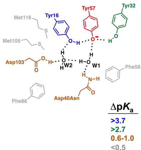
Figure 13. Summary of the effects of Ala mutations on the Tyr57 pK a . Ionized Tyr57 is red, and the residues are colored according to the change in the Tyr pK a value upon mutation of the residue to Ala (ΔpK a , relative to Asp40Asn). The effects at residue 40 are for mutation from Asn to other neutral residues; mutation to charged residue can have larger effects (Tables 9 and 10). Crystallographically observed water molecules are colored black. Mutation of Tyr57 eliminates the observed pK a , as expected (Table 1).
