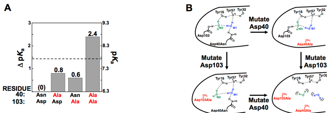
Figure 8. Probing the side chain and water hydrogen-bond network that helps stabilize the ionized Tyr. (A) Effects on the Tyr pK_a for the single Asp40Ala and Asp103Ala mutations and double Asp40Ala/Asp103Ala mutation. The dashed line represents the expected Tyr pK_a if the Ala mutations are additive. The values are from Table 6. (B) Model for the larger than additive effect for mutation of both Asp40 and Asp103 compared to the single mutations. In this model, the water molecules substantially rearrange or become fully mobile only after both mutations are introduced.
