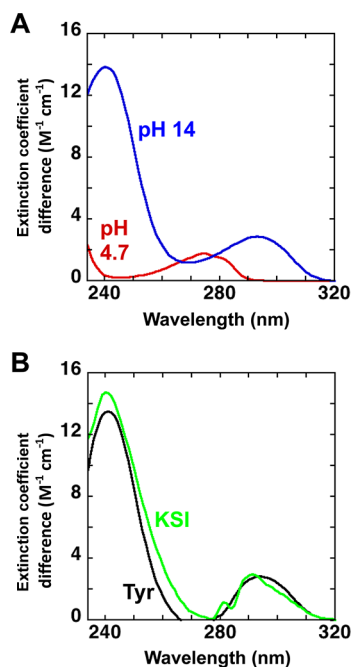
Figure 3. Evaluating tyrosine ionization by UV spectroscopy. (A) Absorbance spectra of tyrosine measured in 10 mM sodium acetate, pH 4.7 (red), and 1 M NaOH, pH 14 (blue). (B) Difference absorbance spectra for tyrosine (pH 14 – pH 4.7, black) and Asp40Asn KSI (pH 10 – pH 4, green). The difference spectra show maxima for tyrosine at 244 ( \Delta\epsilon = 1.3 \times 10^4 \text{ M}^{-1} \text{ cm}^{-1} ) and 295 nm ( \Delta\epsilon = 2.8 \times 10^3 \text{ M}^{-1} \text{ cm}^{-1} ) and for Asp40Asn KSI at 244 ( \Delta\epsilon = 1.4 \times 10^4 \text{ M}^{-1} \text{ cm}^{-1} ) and 293 nm ( \Delta\epsilon = 2.6 \times 10^3 \text{ M}^{-1} \text{ cm}^{-1} ). The similar spectra shape and extinction coefficient differences provide support for the ionization of one tyrosine. The dashed line in Figures 4 and 10 represent the expected extinction coefficient change for the ionization of one tyrosine (green).
